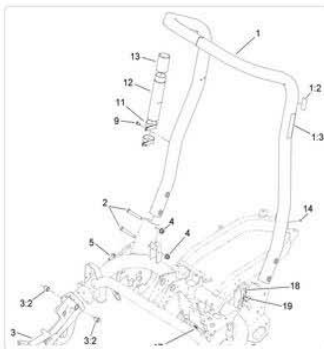
Roll-Over Protection System Assembly
