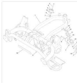
Frame Assembly
